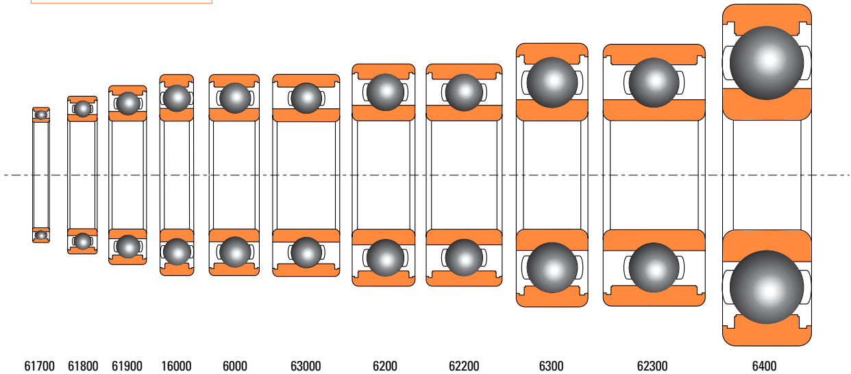
Fig. 4. Timken deep groove ball bearing series.
