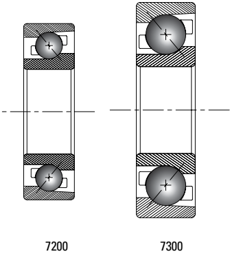
Fig. 17. Single-row angular contact ball bearing series.
