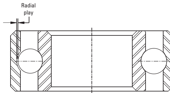
Fig. 16. Radial play.
