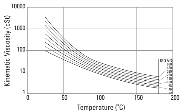
Fig. 50. Temperature vs. kinematic viscosity.
