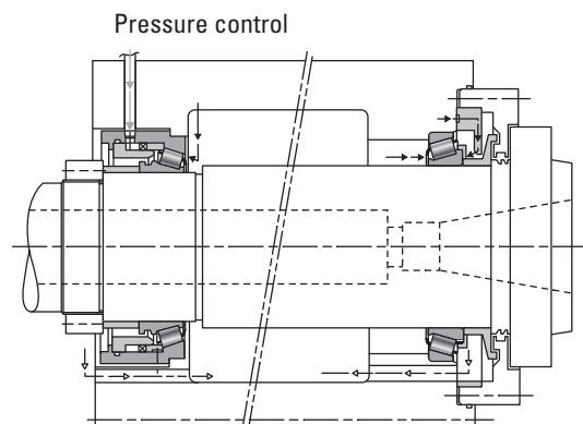
Fig. 80. Simple mounting with a Hydra-Rib bearing cooled by an axial oil inlet and a TSMA bearing with oil jets at both ends of the rollers for inlet and cooling.
