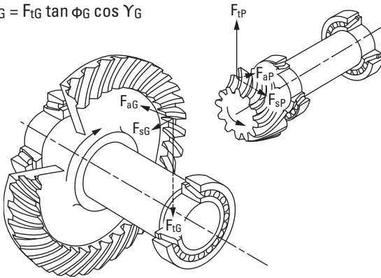
Fig. 39. Straight bevel gearing.
