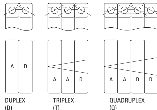
Fig. 120. Ball screw support bearing mounting configurations.
