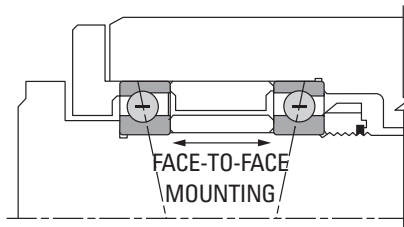
Fig. 87. DF Mounting, fixed (not suggested).
