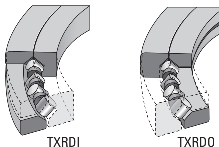
Fig. 11. TXRDI and TXRDO.
