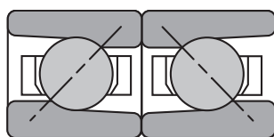
Back-to-Back DB
