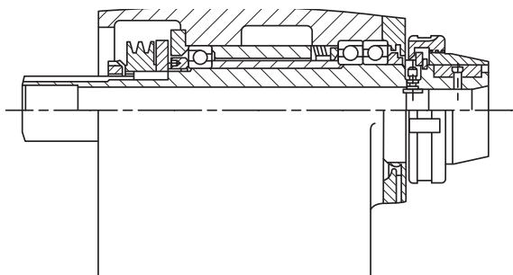
Fig. 133. Super precision lathe headstock.
