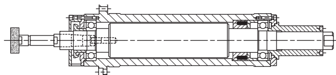
Fig. 122. High-speed internal-grinding spindle.
