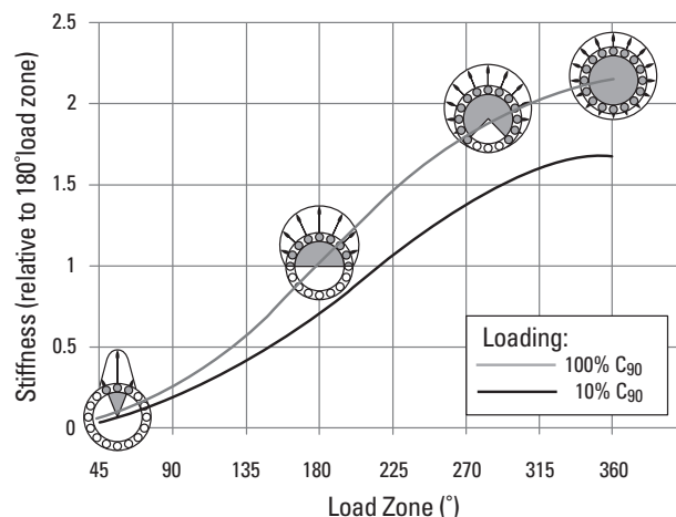
Fig. 5. Effect of load zone on bearing stiffness.
