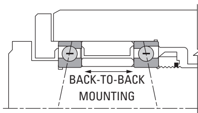
Fig. 88. DB Mounting, fixed (suggested).
