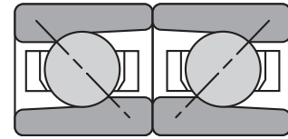
Face-to-Face DF
