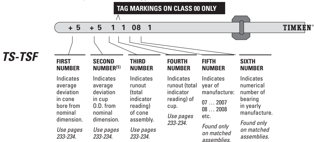
Fig. 102. Inch system precision bearing tag markings.
