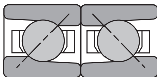
Back-to-Back DB
