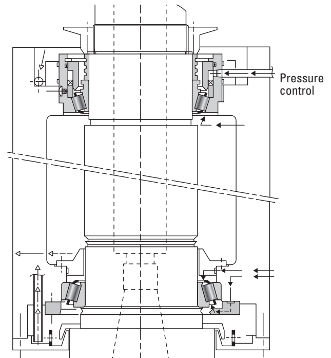
Fig. 65. Typical example of proper use of an oil-lubricated vertical axis spindle with pressure control for the oil and a means to collect and extract the oil.
