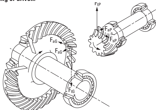
Fig. 41. Spiral bevel and hypoid gearing.
