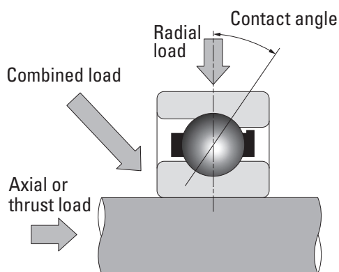
Fig 14. Example of ball bearing loading.
