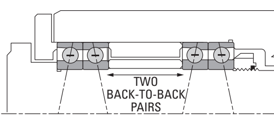
Fig. 88. DB Mounting, fixed (suggested).
