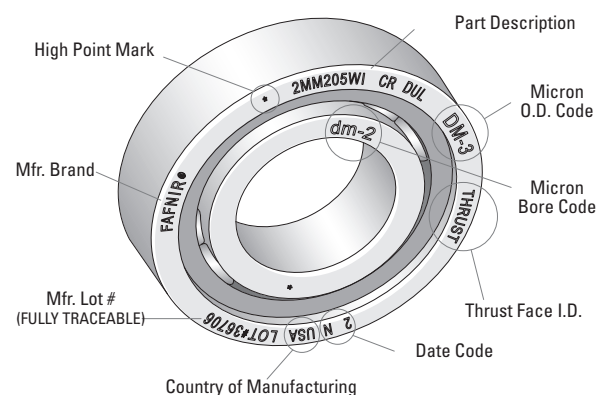
Fig. 121. Super precision markings.
