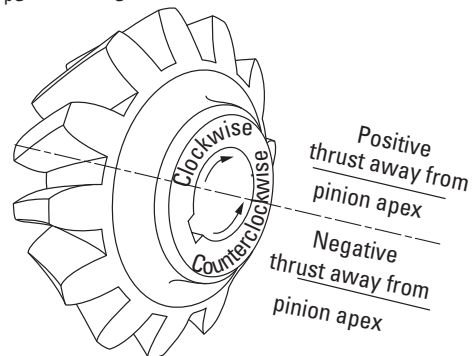
Fig. 40 Spiral bevel and hypoid gears – the direction of thrust and separating forces depends upon spiral angle, hand of spiral, direction of rotation, and whether the gear is driving or driven.
