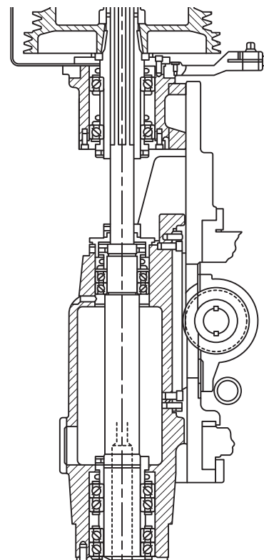
Fig. 135. Precision vertical milling spindle.
