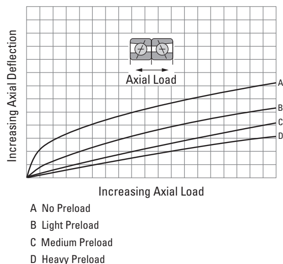
Fig. 96. Effect of most commonly used preloads on axial deflection.
