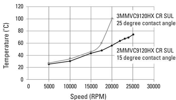
Fig 17. Effect of contact angle on temperature.
