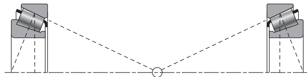
Fig. 93. Graphical determination of optimum thermal spread.
