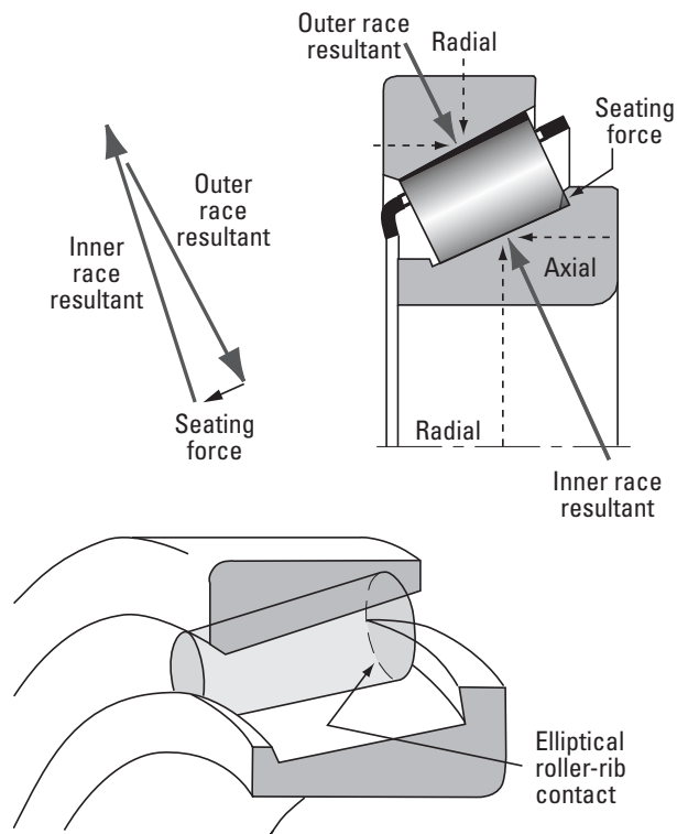
Fig. 10. Small seating force from the inner race rib keeps rollers aligned on the raceway.
