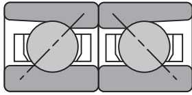
Back-to-Back DB
