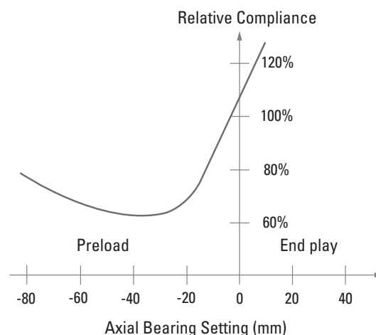
Fig. 31. Effect of bearing setting on spindle system dynamic stiffness.
