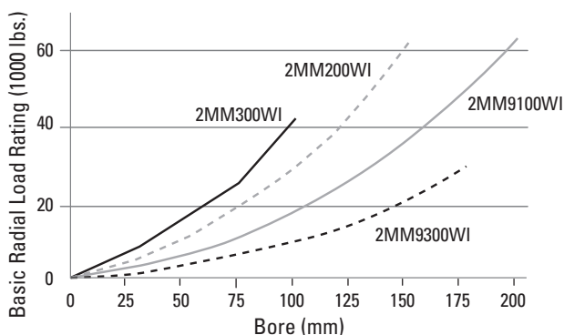
Fig 21. Angular contact ball bearing load ratings.
