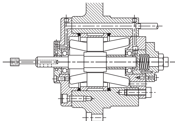
Fig. 131. 100000 RPM high-cycle wheelhead.
