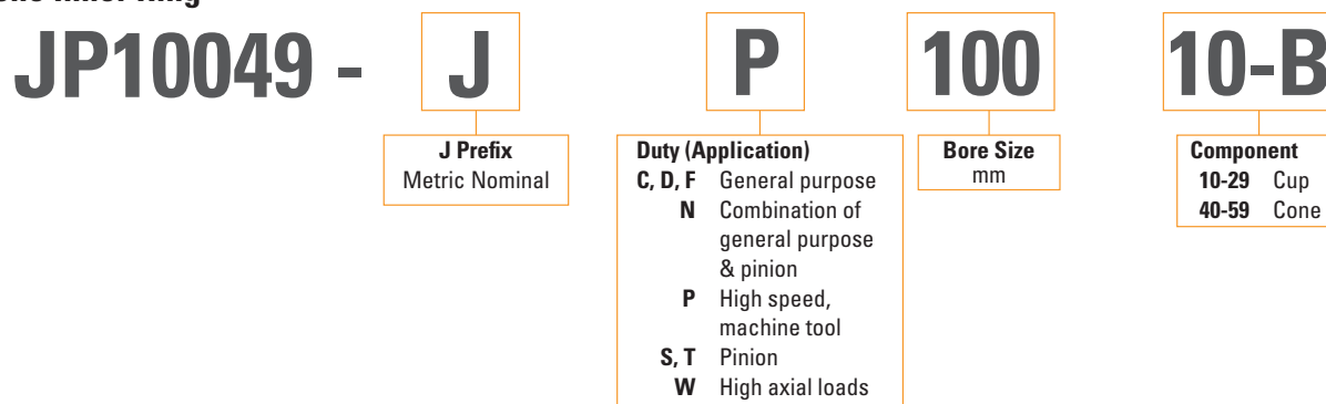
Fig 99. Precision tapered roller bearing ISO 355 nomenclature.
