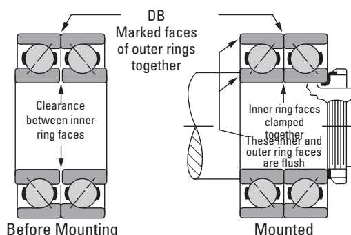
Fig. 83. Back-to-back bearing assemblies before and after mounting.
