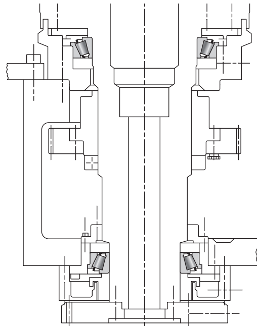
Fig. 64. Vertical axis spindle.
