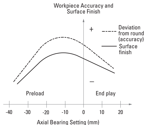
Fig. 32. Effect of bearing setting on surface finish and accuracy of the workpieces.
