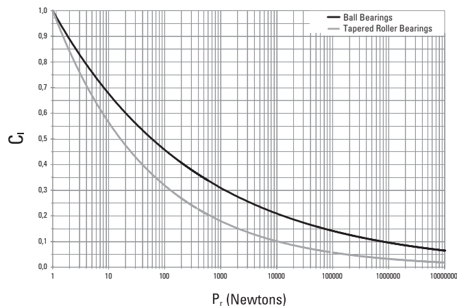
Fig. 47. Load factor ( C_l ) vs. equivalent bearing load ( P_r ).
