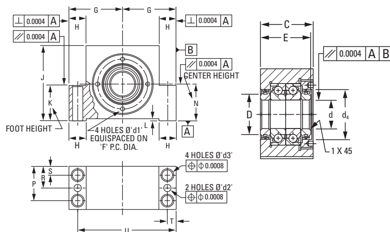
HEAVY-DUTY SERIES – DIMENSIONAL TOLERANCES \pm 0.13 \text{ mm} ( \pm 0.005 \text{ in.} ) UNLESS OTHERWISE STATED.
