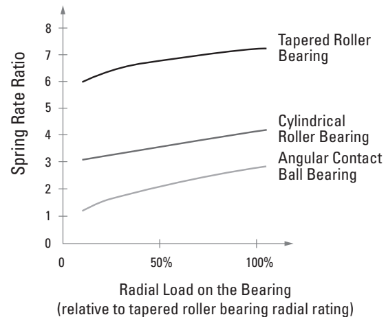
Fig. 28. Radial spring rate comparison between popular machine tool bearings of a comparable size under zero internal clearance.
