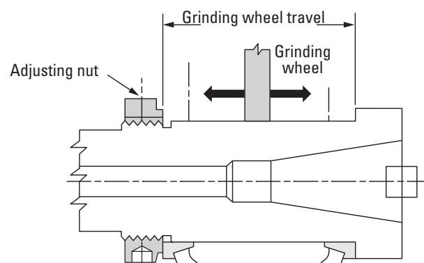
Fig. 73. Grinding of cone shaft and backing shoulders.
