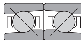
Face-to-Face DF
