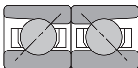
Back-to-Back DB
