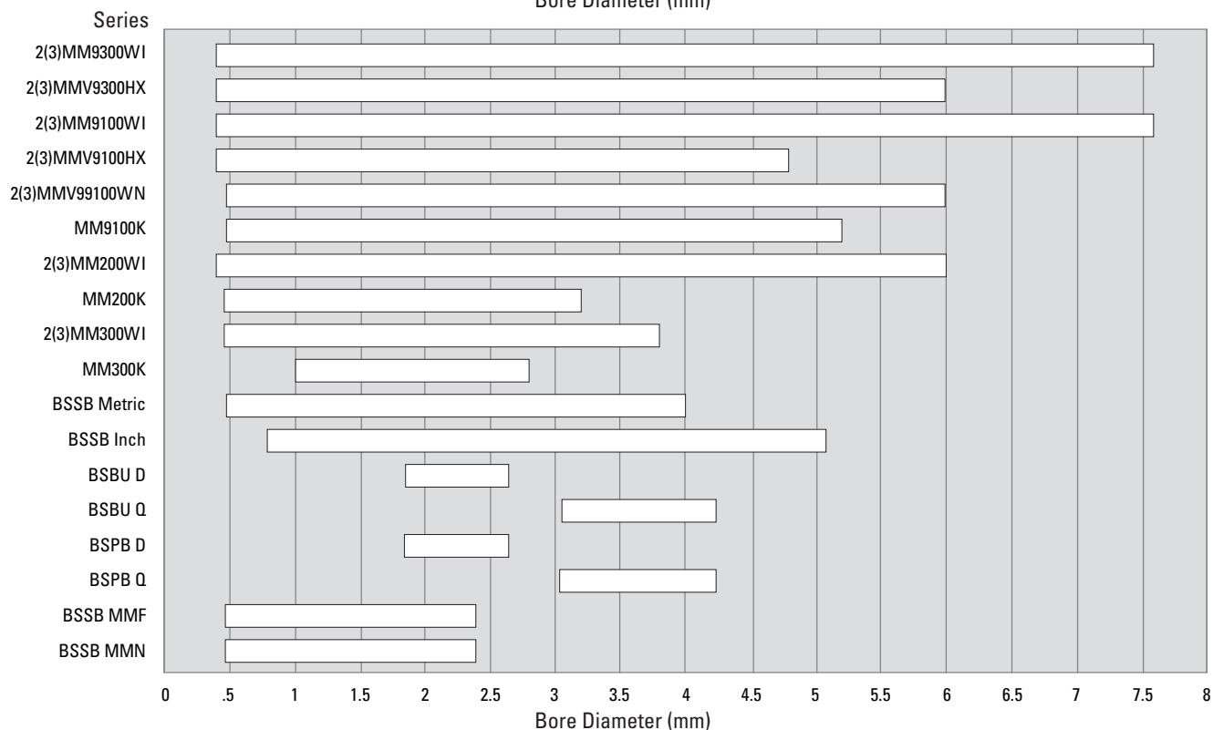
Fig. 136. Bore diameters.
