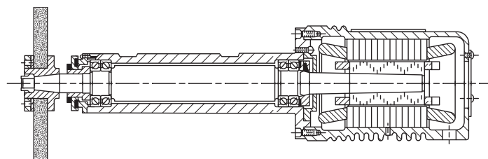
Fig. 124. Precision surface-grinding spindle.
