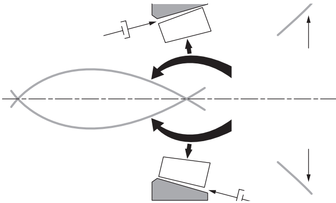
Fig. 33. Damping in a tapered roller bearing.
