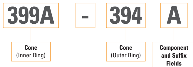
Fig 98. Precision tapered roller bearing nomenclature.
