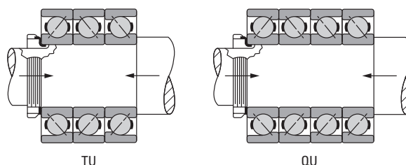
Fig. 86. Typical triplex and quadruplex bearing mountings.
