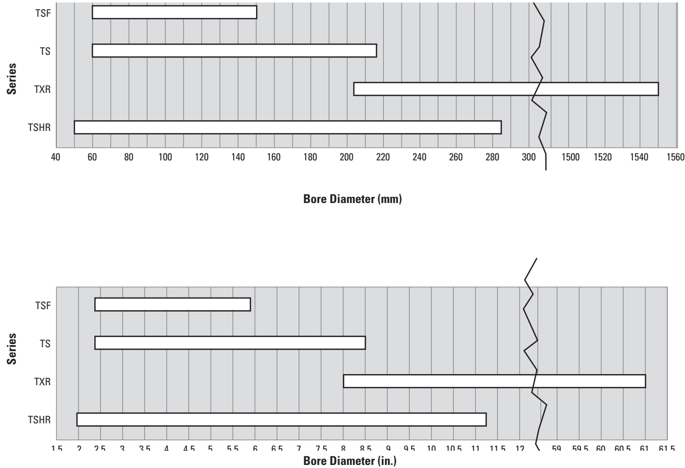
Fig. 109. Bore diameters.
