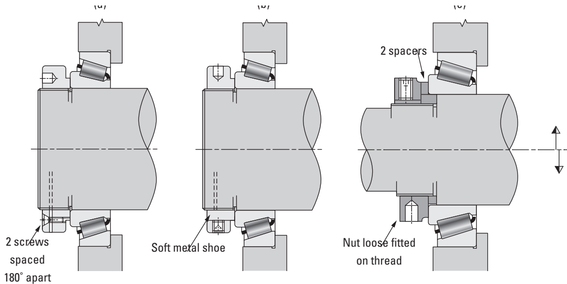
Fig. 71. Locking devices.
