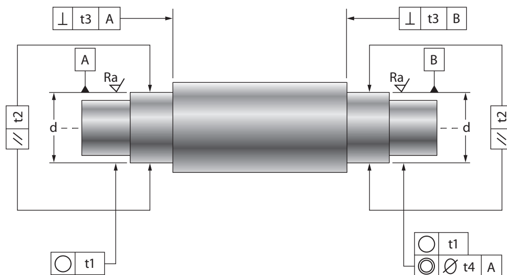
Fig. 69. Shaft Tolerances.
