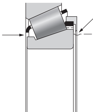
Fig. 60. The TSMA bearing.
