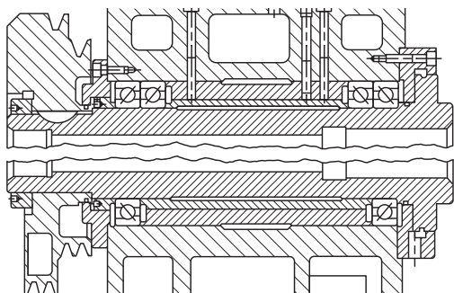
Fig. 128. Ultra-precision grinding workhead.
