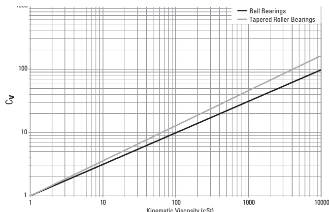
Fig. 51. Viscosity factor ( C_v ) vs. kinematic viscosity.
