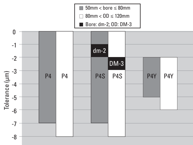
Fig. 6. Tolerance spreads of a bearing with a bore micron code of dm-2 and an O.D. micron code of DM-3.
