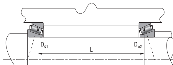
Fig. 94. Resulting distance between bearing geometric centerlines.
