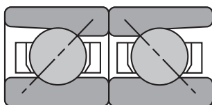
Back-to-Back DB
