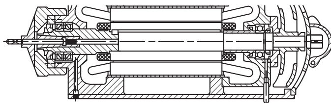
Fig. 134. High-speed motorized router.
