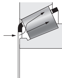
Fig. 54. Pumping effect of a tapered roller bearing.
