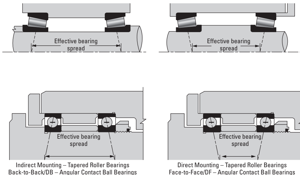
Fig. 35. Choice of mounting configuration for single-row bearings, showing position of effective load-carrying centers.
