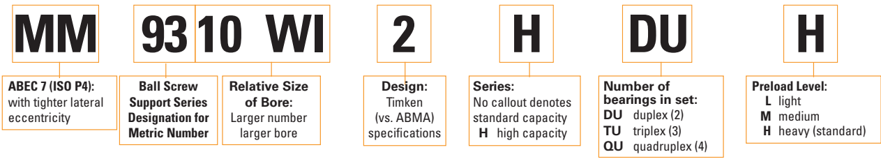
Fig. 113. Super precision ball bearing, ball screw support, single-row nomenclature - inch.
