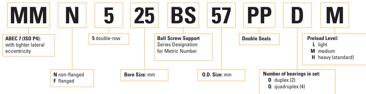
Fig. 114. Super precision ball bearing, ball screw support, double-row nomenclature - metric.
