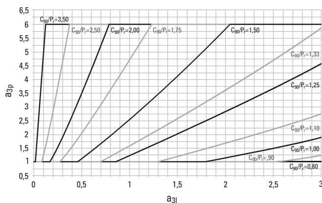
Fig. 52. Low load factor ( a_{3p} ) vs. lubricant life factor ( a_{3l} ) and C_{90}/P_f ratio.
