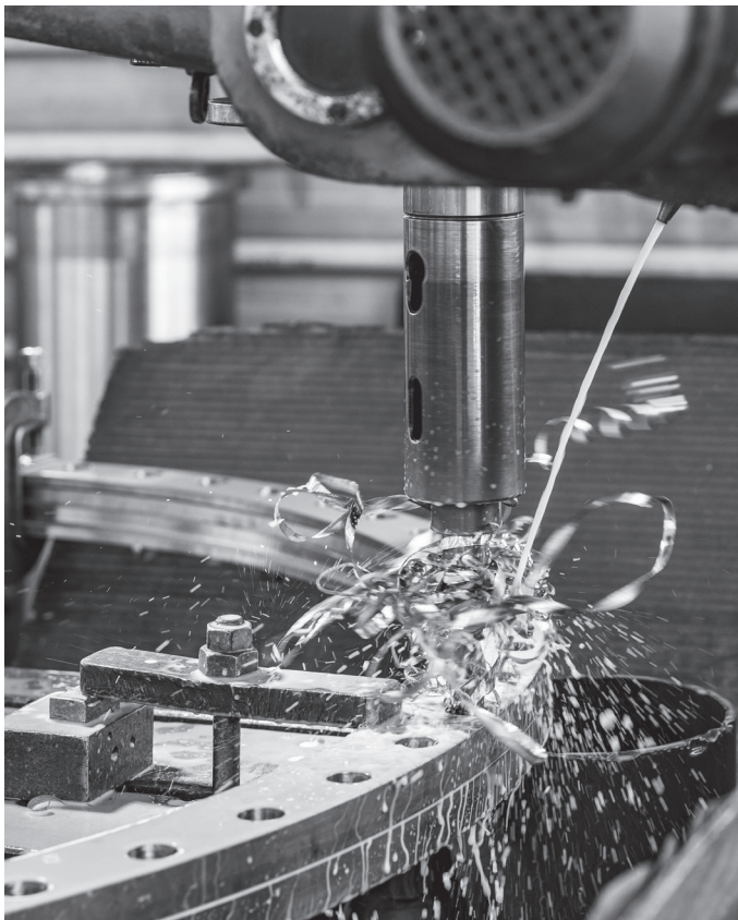
Fig. 64. Vertical axis spindle.
