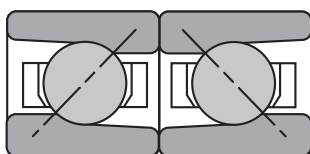
Back-to-Back DB
