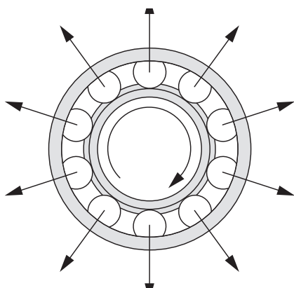
Fig 15. Centrifugal forces of a rotating ball bearing.
