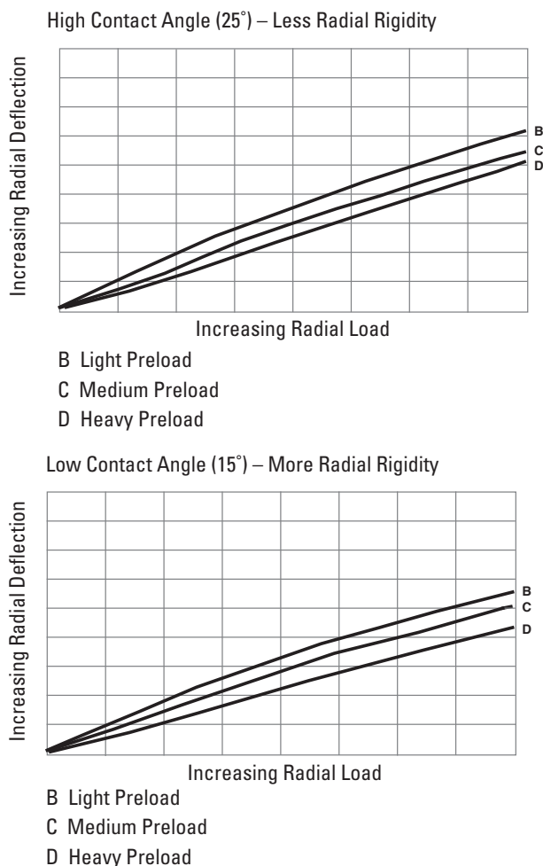
Fig. 19. Effect of contact angle on radial deflection.
