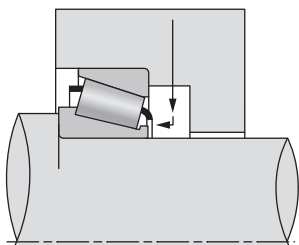
Fig. 58. Axial oil jet to direct oil at small end of the rollers.
