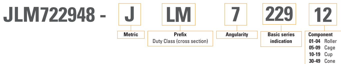
Fig 100. Precision tapered roller bearing ABMA nomenclature.
