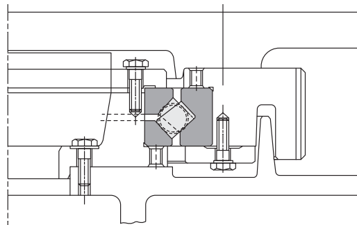
Fig. 81. Typical mounting arrangement of a TXRDO bearing.
