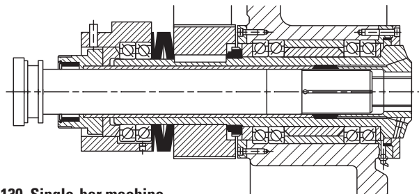
Fig. 130. Single-bar machine.
