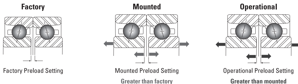
Fig. 23. Preload settings.
