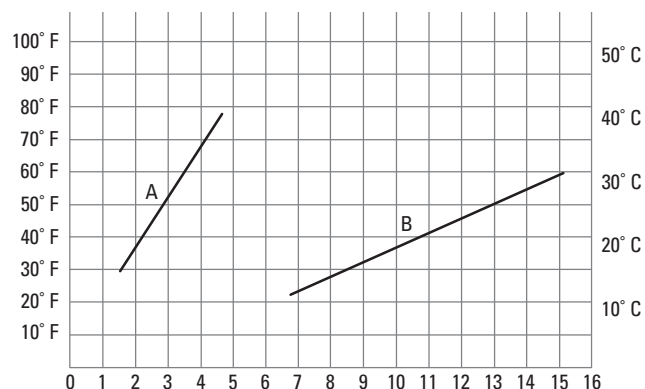
Fig. 67. Effect of preload on temperature rise.
