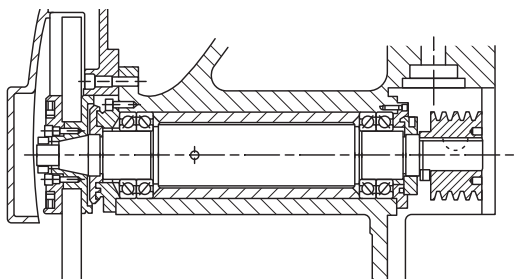
Fig. 129. Precision toolroom surface grinder spindle.
