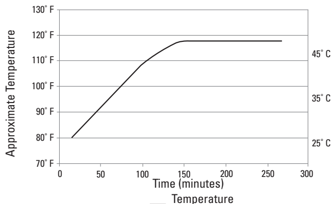
Fig. 63. Typical temperature after break-in procedure.
