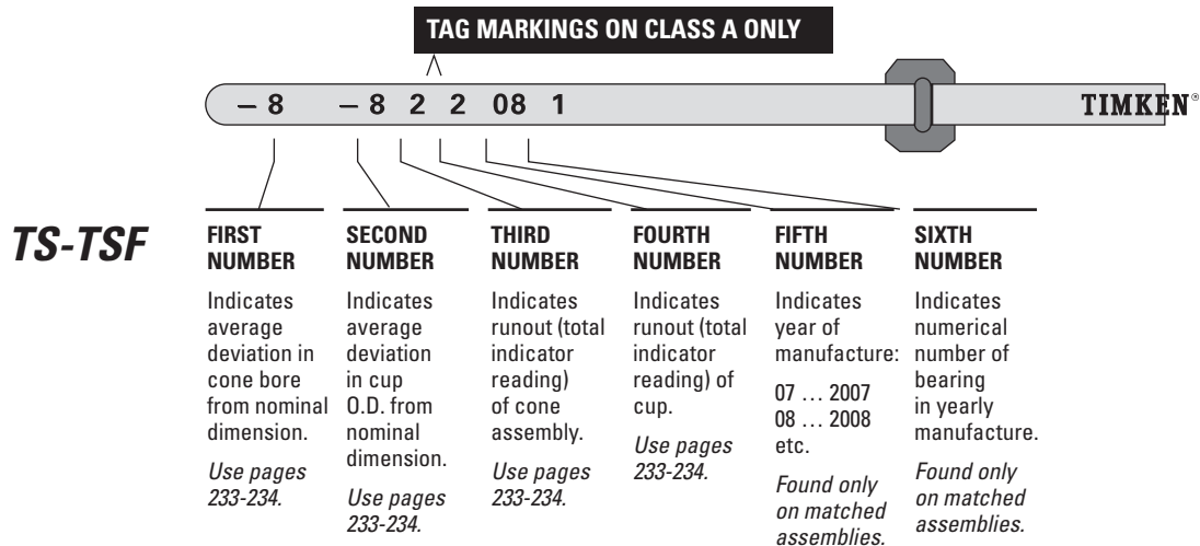
Fig. 101. Metric system precision bearing tag markings.
