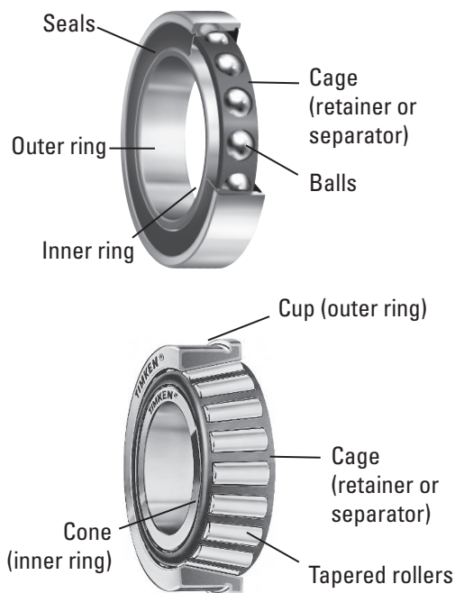
Fig. 2. Bearing components.
