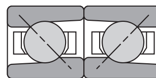
Face-to-Face DF
