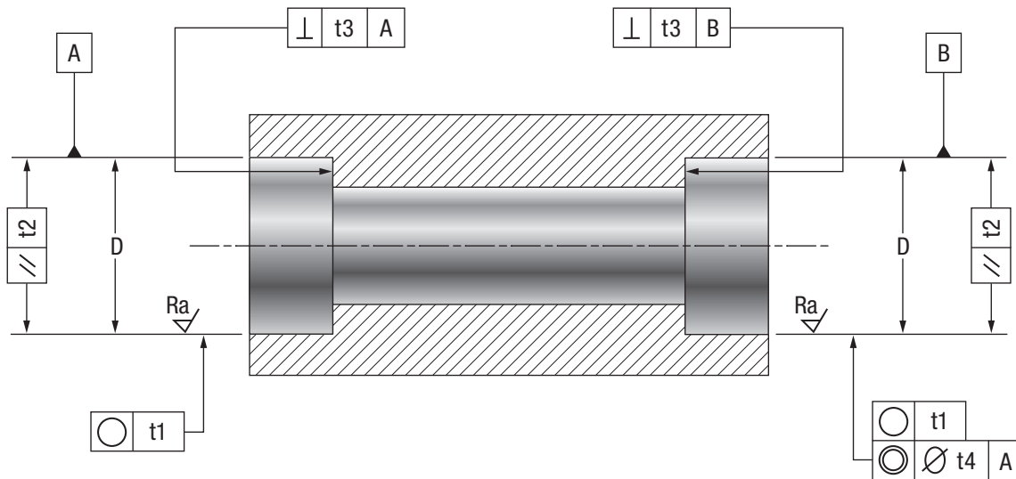
Fig. 70. Housing Tolerances.
