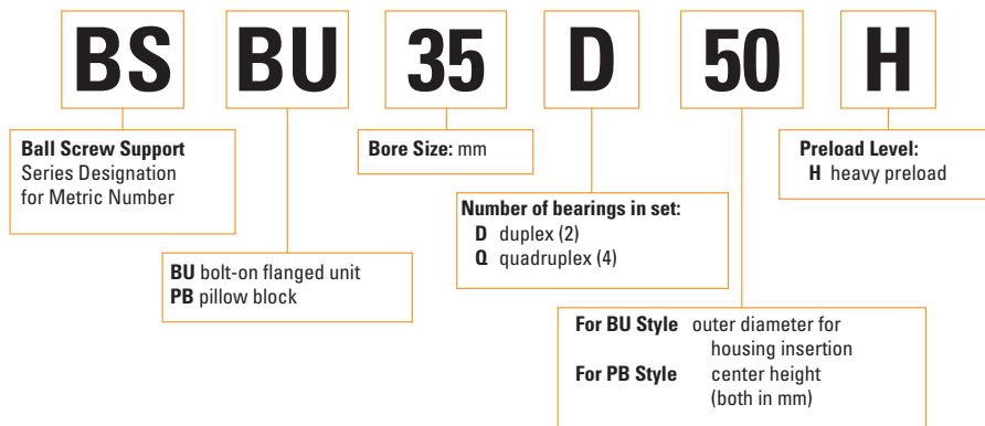
Fig. 115. Super precision ball bearing, ball screw cartridge units nomenclature - metric.
