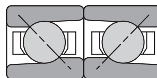
Face-to-Face DF
