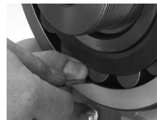
Fig. 15. During mounting, the RIC should be checked at the unloaded roller.
