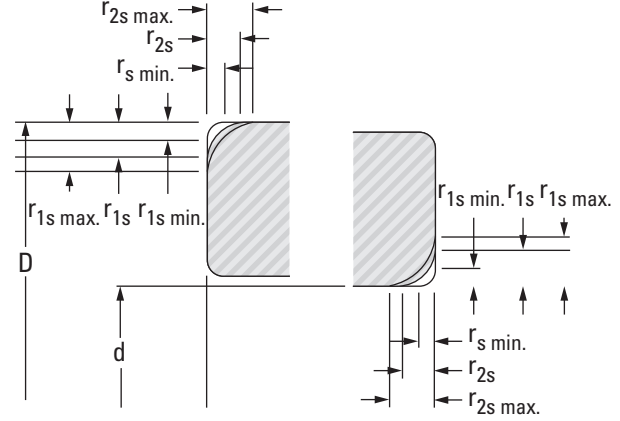
Thrust Bearings
