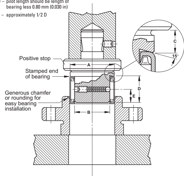
Fig. B2-14. Installation of open ends full complement bearings
