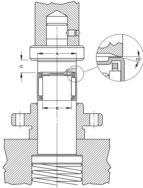
Fig. B2-3. Installation of closed end caged bearings
