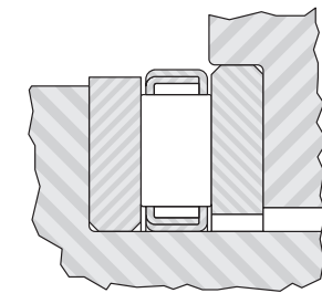
Fig. B6-7. Typical mounting of a thrust bearing when the shaft rotates
