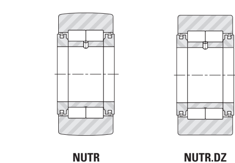
Fig. B5-11. Yoke-type track rollers with end washers, full complement of cylindrical rollers
