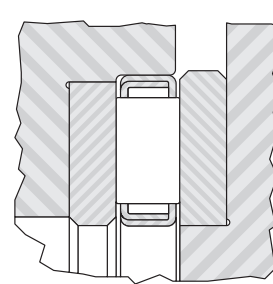
Fig. B6-8. NTHA possible mounting arrangement
