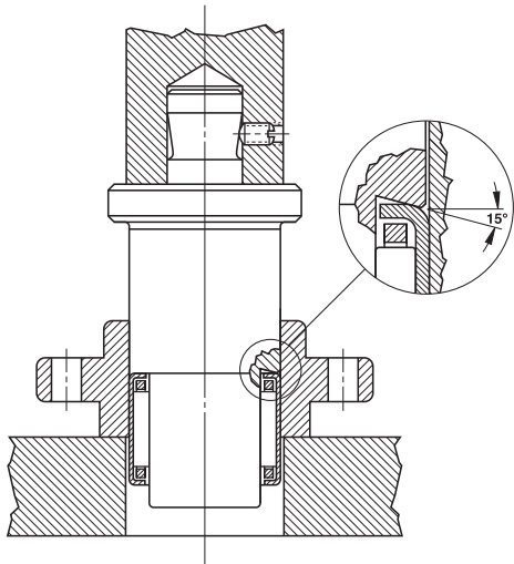
Fig. B2-4. Extraction from a straight housing
