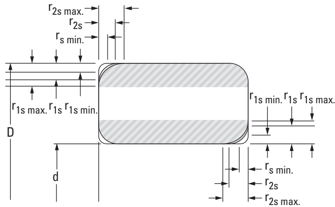
Radial Bearings
