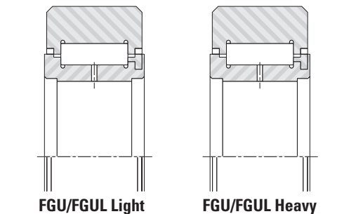
Fig. B5-9. Yoke-type track rollers with metal seals, full complement of cylindrical rollers
