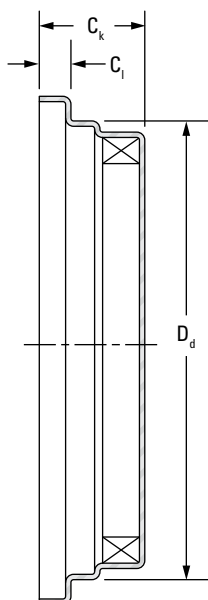
Seal Case
