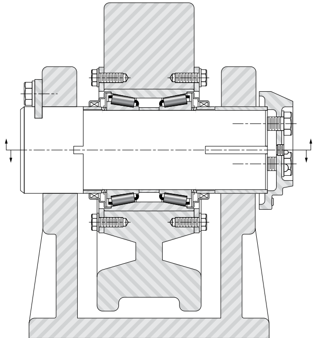
Fig. 23 Furnace wheel
