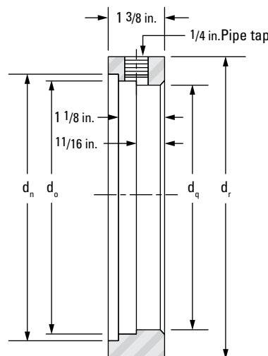
Backing Spacer
