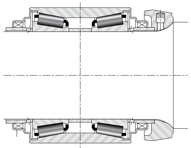
Fig. 21b Cross section of AP bearing in coal crusher
