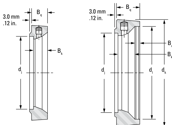
Backing Rings Without Shroud
