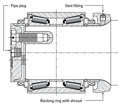
Fig. 49 Mounting Arrangement 6
