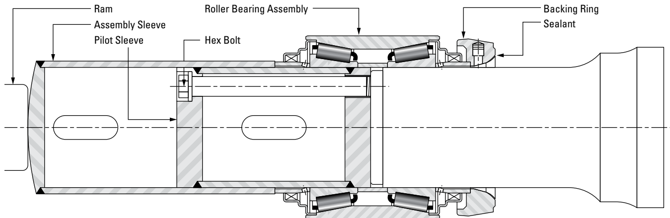
Fig. 26 Separate sleeve method of applying roller bearings to a shaft
