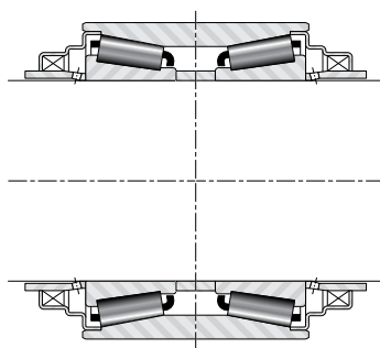
Fig. 43 Mounting Arrangement 4
