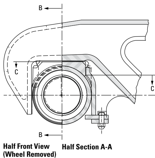
Fig. 19 Mounted adapter
