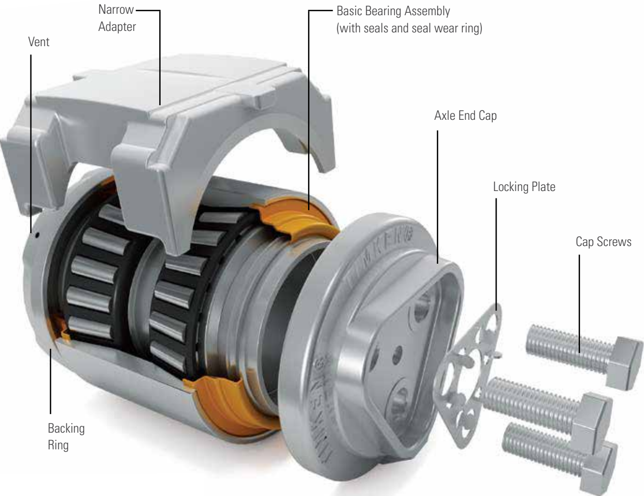
Fig. 33 3D illustration of AP bearing
