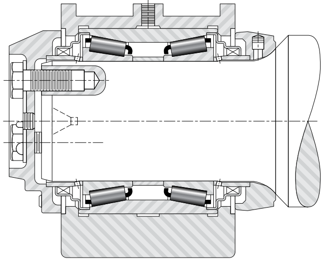
Fig. 22b Cross section of wood pulp beater spindle
