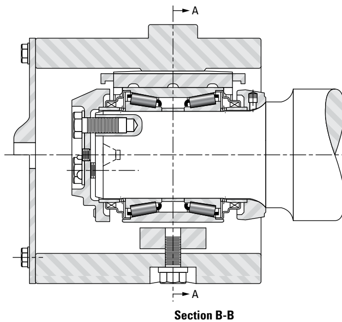
Fig. 16 Cross section of AP bearing in ingot car
