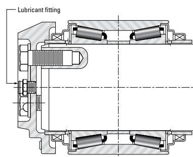
Fig. 39 Mounting Arrangement 3
