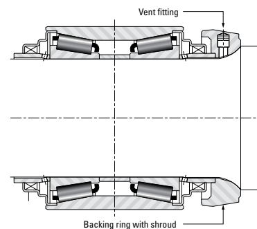
Fig. 36 Mounting Arrangement 2
