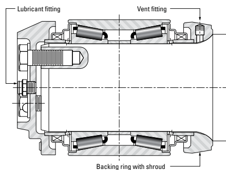
Fig. 34 Mounting Arrangement 1
