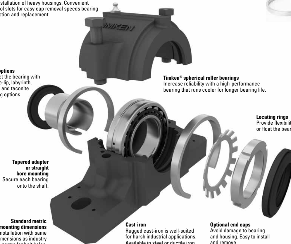
Fig. E-13. SNT plummer block components and features.
