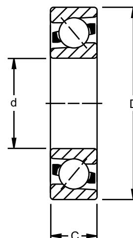
7412WN and 7415WN MBR 40° Contact Angle
