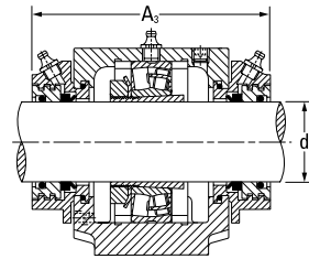
Taconite Seal
