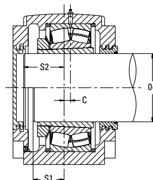
MINIMUM AND MAXIMUM SHAFT LENGTHS 3000 SERIES
