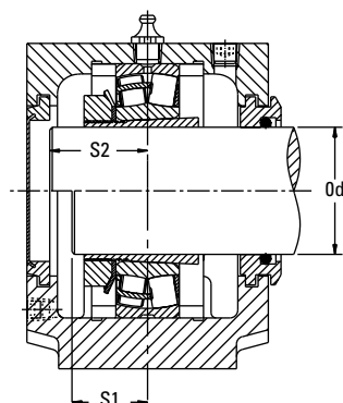
MINIMUM AND MAXIMUM SHAFT LENGTHS 500/600 AND 200/300 SERIES – 2 AND 4 BOLT
