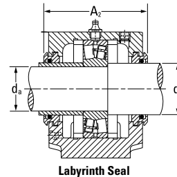
Labyrinth Seal
