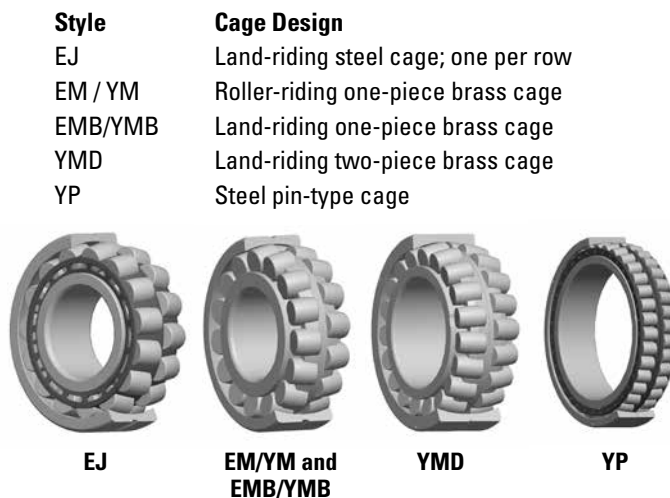
Fig. 35. Radial spherical roller bearings.
