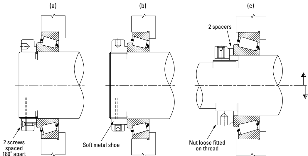
Fig. 113. Locking devices.
