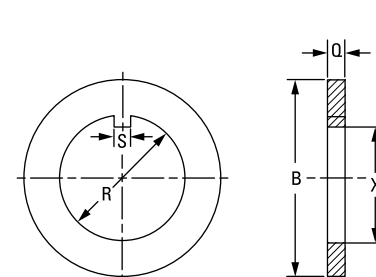
Fig. 51. Tongued washers.
